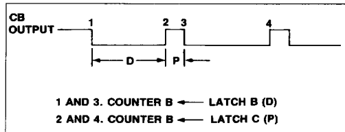
Figure 6-5. Counter B Pulse Generation
