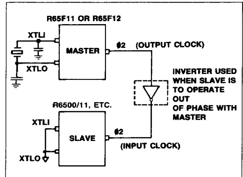
Figure 3-4. Master/Slave Connections
