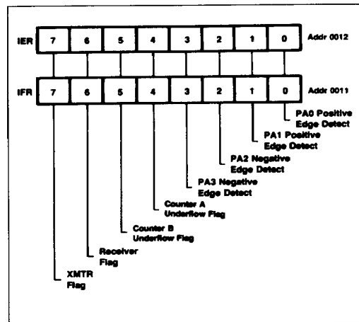
Figure 3-6. Interrupt Enable and Flag Registers
