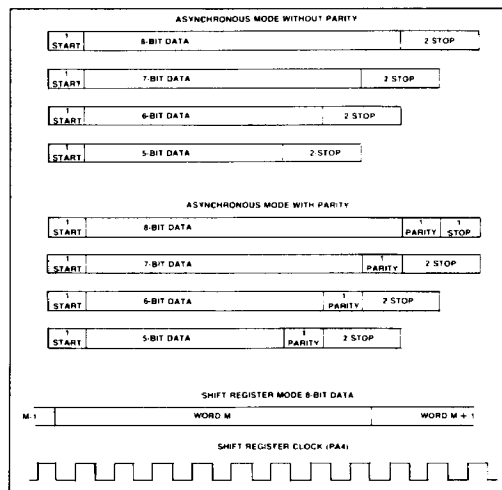
Figure 5-2. Bit Allocations
